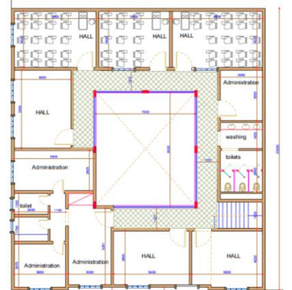
typical floor
